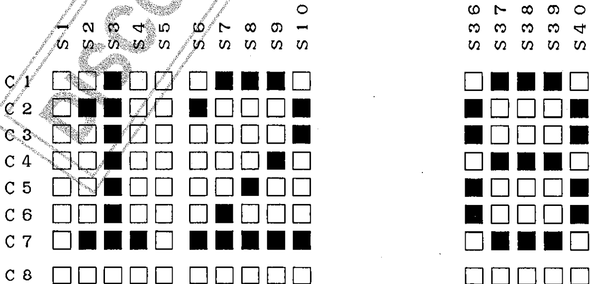
Common driver pins, segment driver pins and character display
